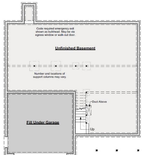
Basement Plan
